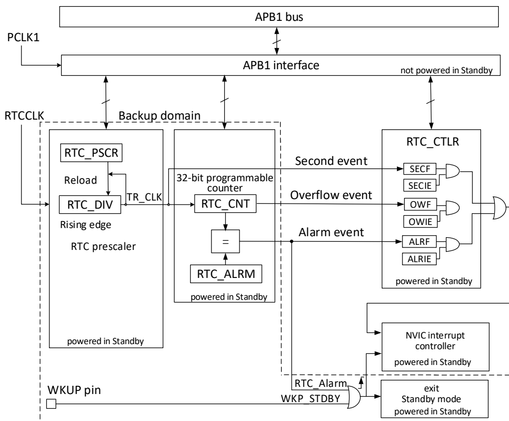
Figure 6-1 RTC structure diagram
