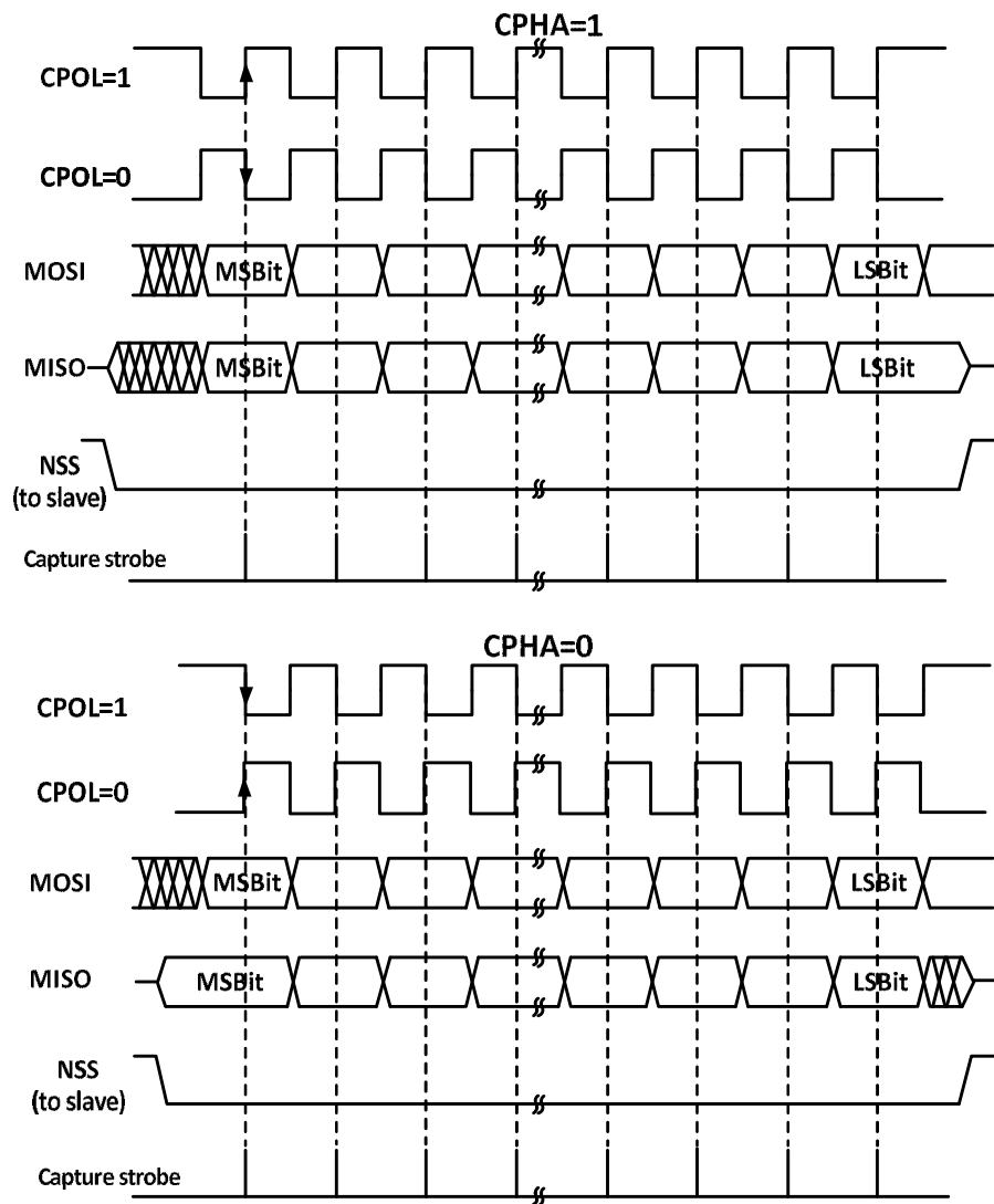
Figure 19-2 SPI model
