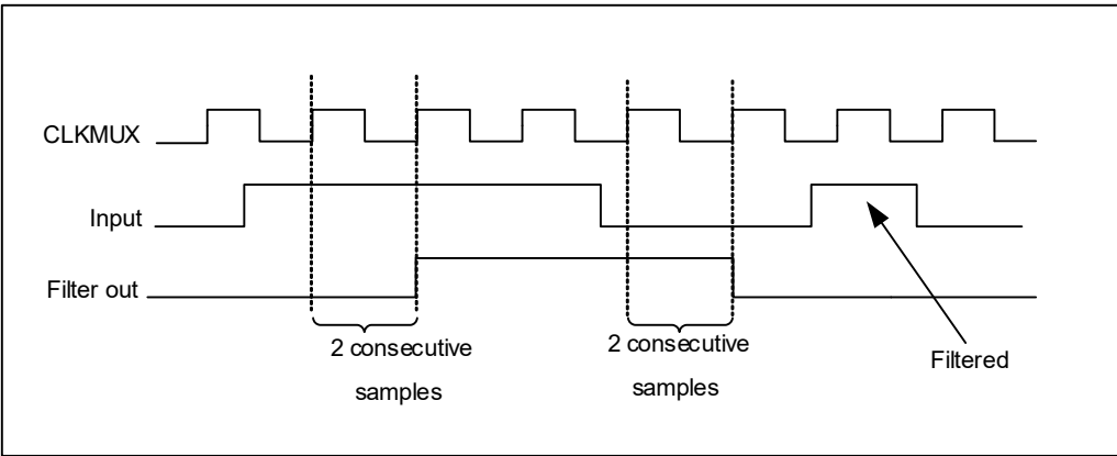
Figure 16-2 Timing block diagram of interference filter
