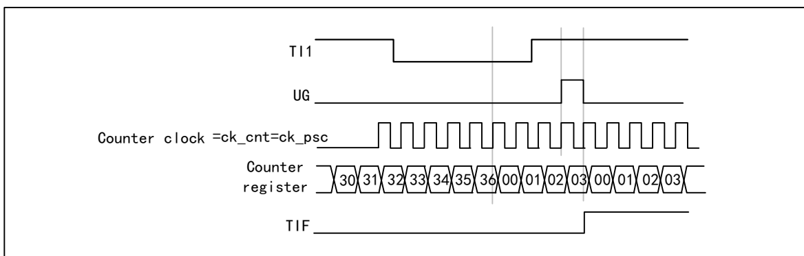
Figure 14-6 Control circuit in reset mode
