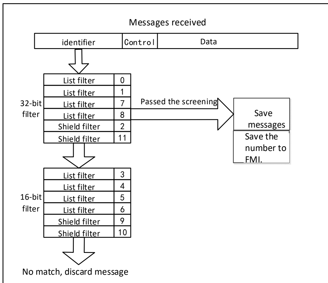
Figure 22-5 Filter example
